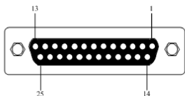
DB25Female/hole)
