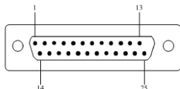
DB25Male/needle)
