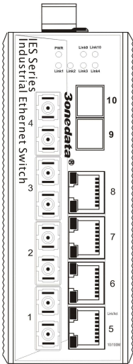
Front Panel
