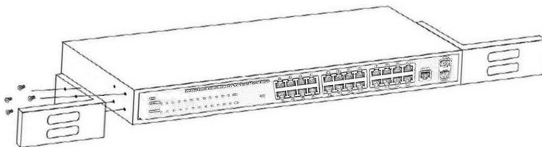
Figure 5 - Bracket Installation
